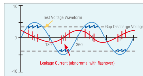
Flashover Waveform
